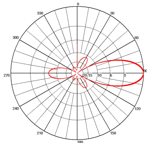
Vertical diagram (E plane)
