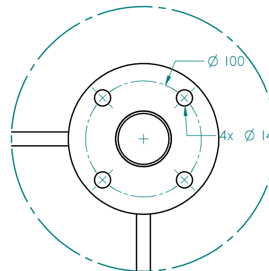
DETAIL A
